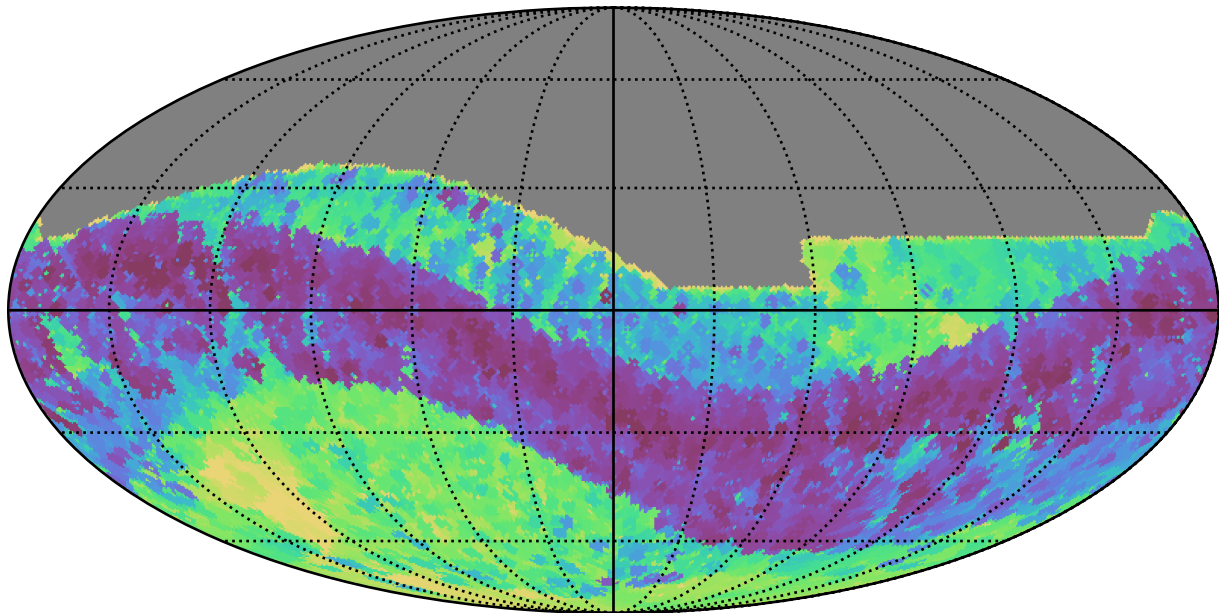
ddf_half_v3.4_10yrs All sky z band: Min skyBrightness
