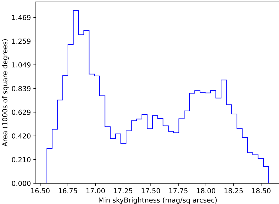
ddf_half_v3.4_10yrs All sky z band: Min skyBrightness
