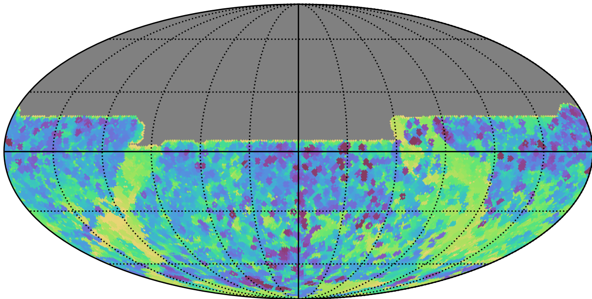
ddf_half_v3.4_10yrs All sky y band: Min skyBrightness
