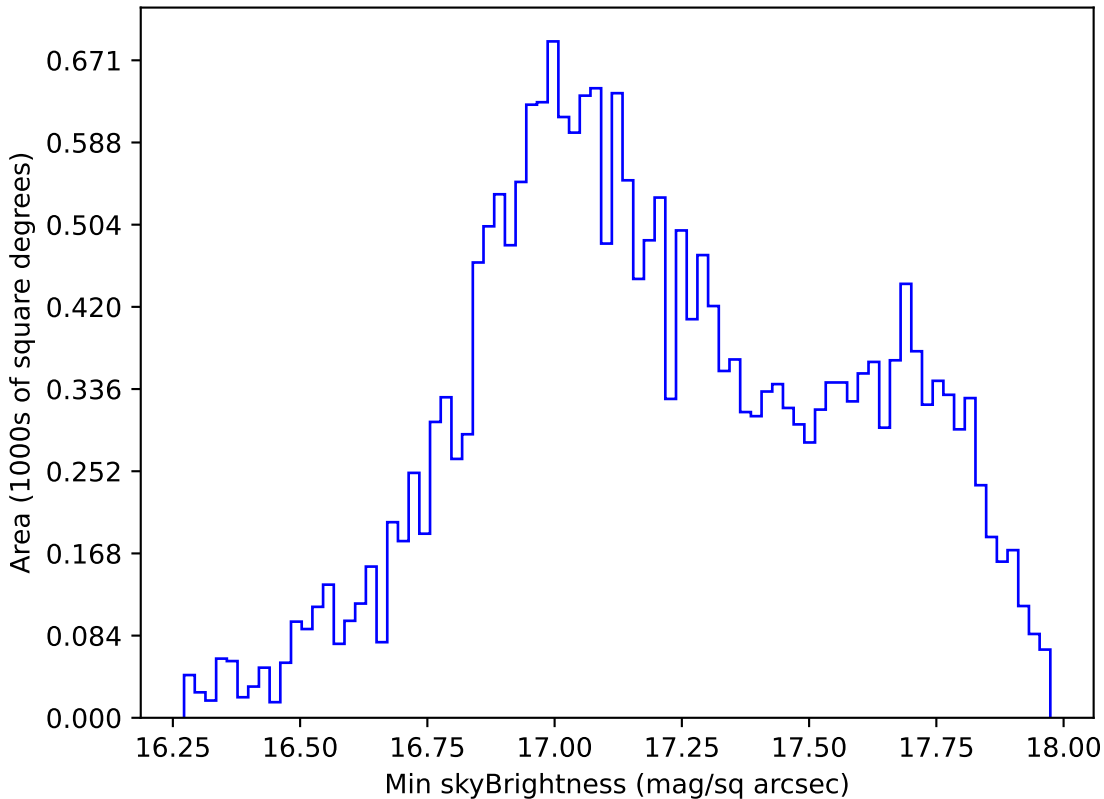
ddf_half_v3.4_10yrs All sky y band: Min skyBrightness
