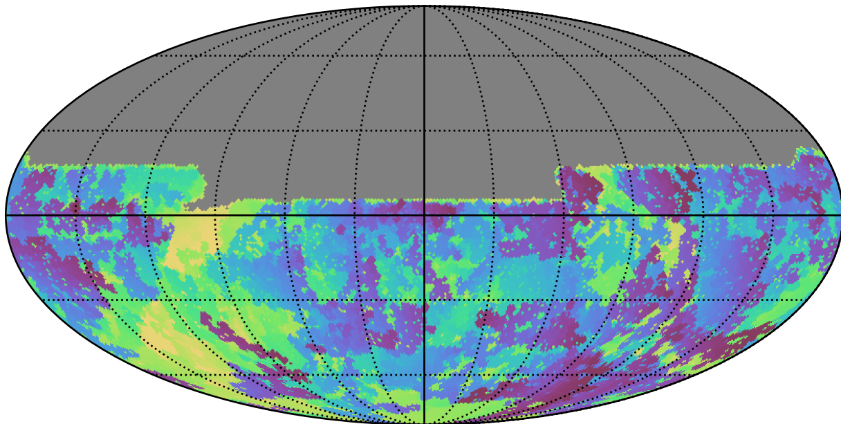
ddf_half_v3.4_10yrs All sky u band: Min skyBrightness
