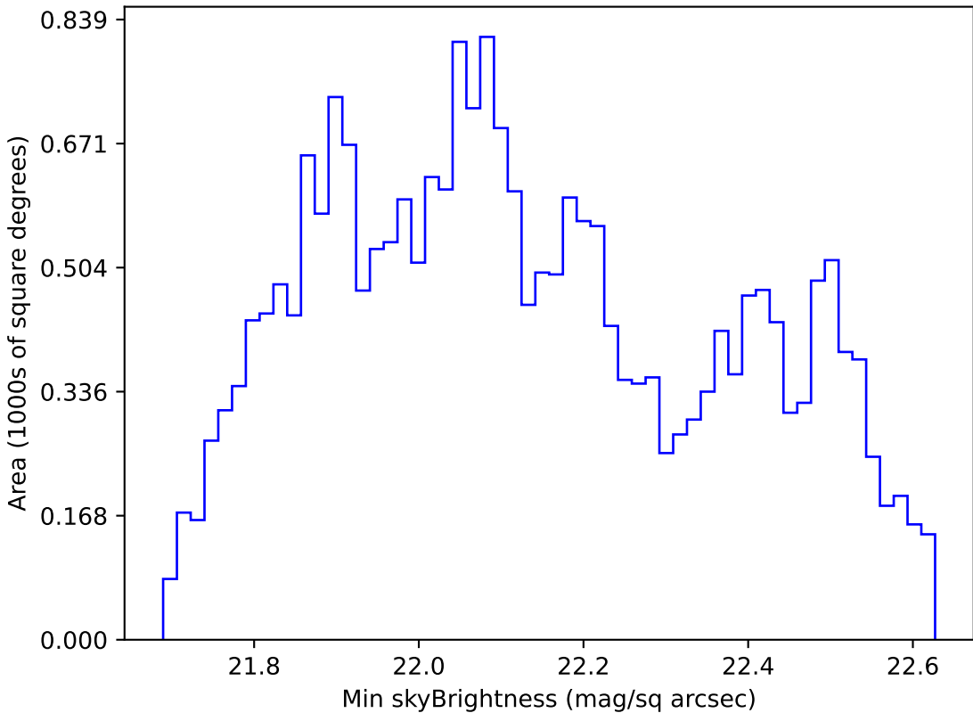
ddf_half_v3.4_10yrs All sky u band: Min skyBrightness
