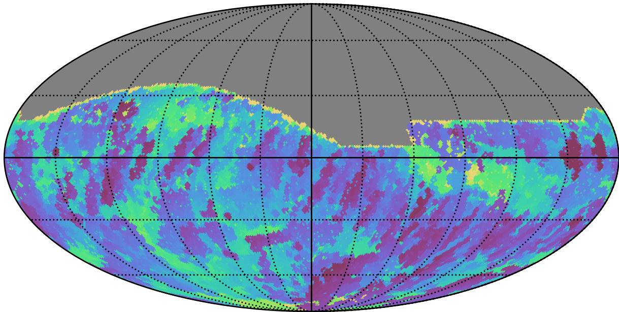
ddf_half_v3.4_10yrs All sky r band: Min skyBrightness
