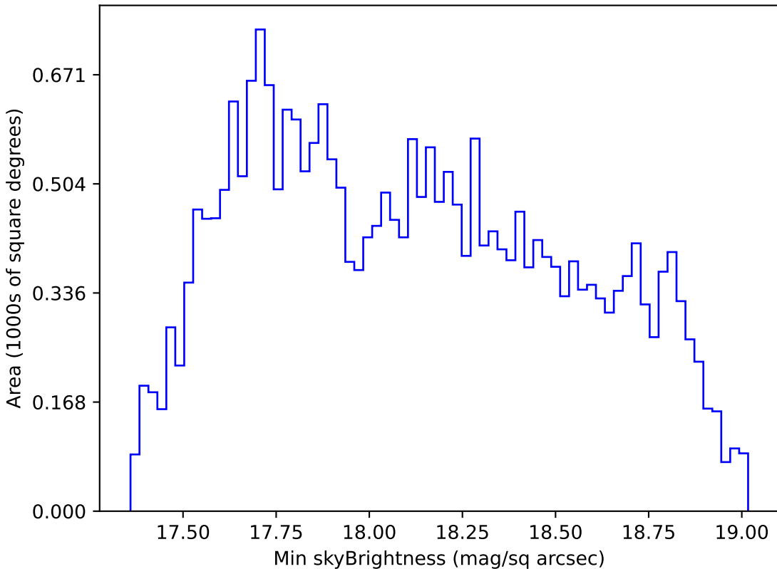
ddf_half_v3.4_10yrs All sky i band: Min skyBrightness
