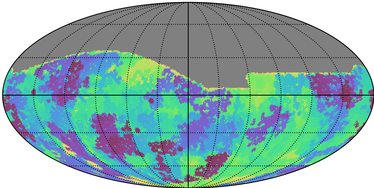
ddf_half_v3.4_10yrs All sky g band: Min skyBrightness
