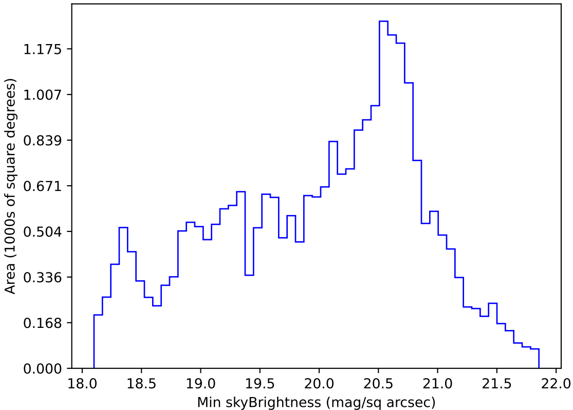
ddf_half_v3.4_10yrs All sky g band: Min skyBrightness
