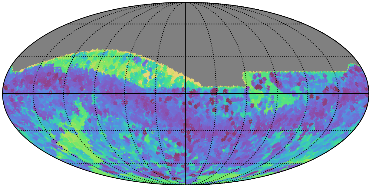
ddf_half_v3.4_10yrs All sky all bands: Min skyBrightness
