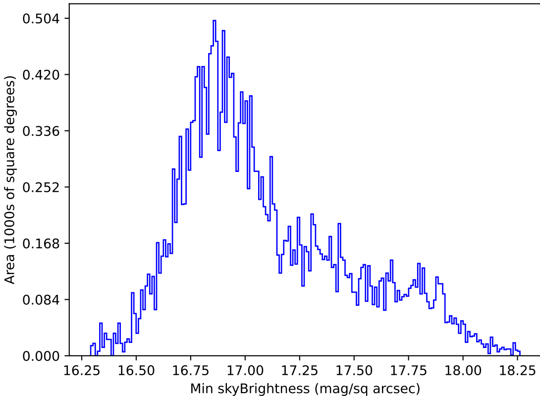
ddf_half_v3.4_10yrs All sky all bands: Min skyBrightness
