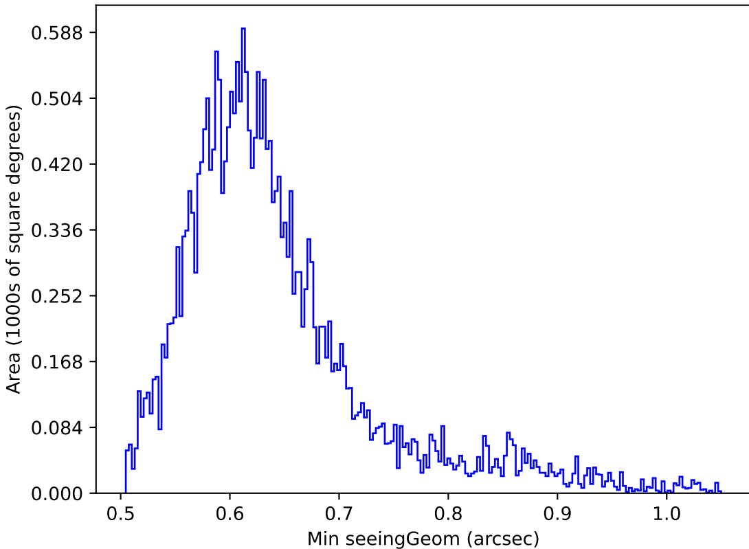
ddf_half_v3.4_10yrs Yr 1 z band: Min seeingGeom
