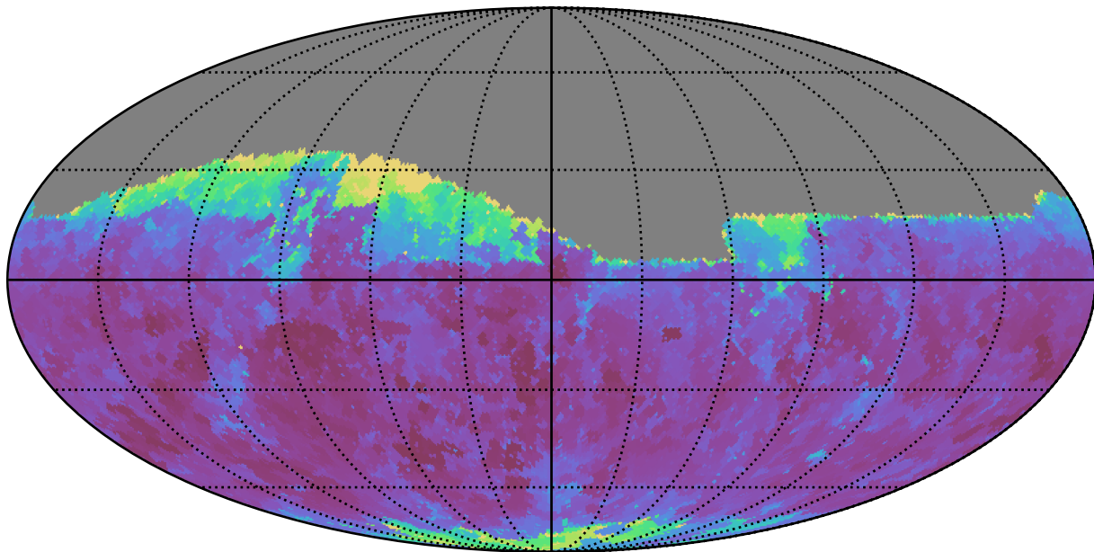
ddf_half_v3.4_10yrs Yr 1 r band: Min seeingGeom
