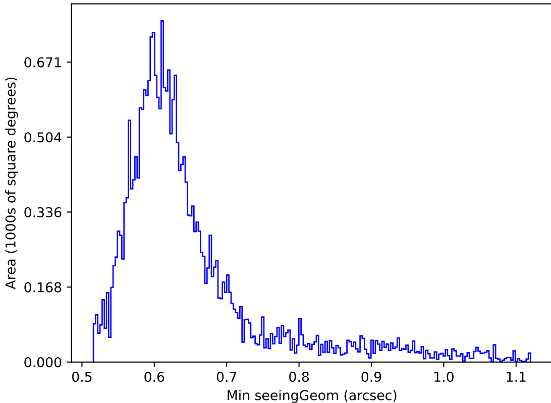
ddf_half_v3.4_10yrs Yr 1 r band: Min seeingGeom
