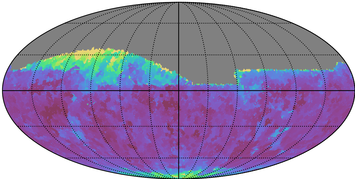
ddf_half_v3.4_10yrs Yr 1 i band: Min seeingGeom
