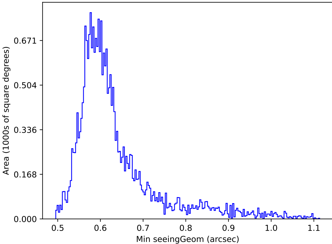
ddf_half_v3.4_10yrs Yr 1 i band: Min seeingGeom
