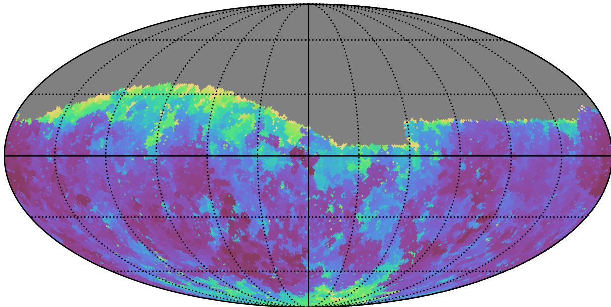
ddf_half_v3.4_10yrs Yr 1 g band: Min seeingGeom
