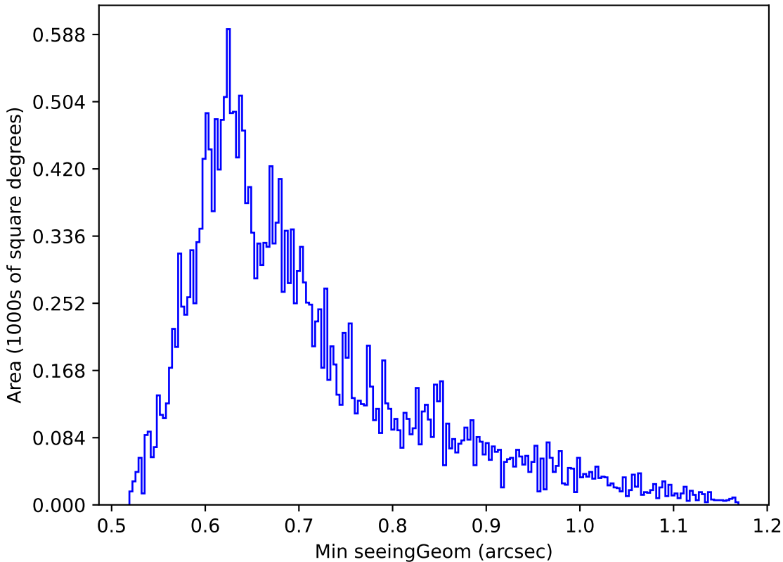
ddf_half_v3.4_10yrs Yr 1 g band: Min seeingGeom
