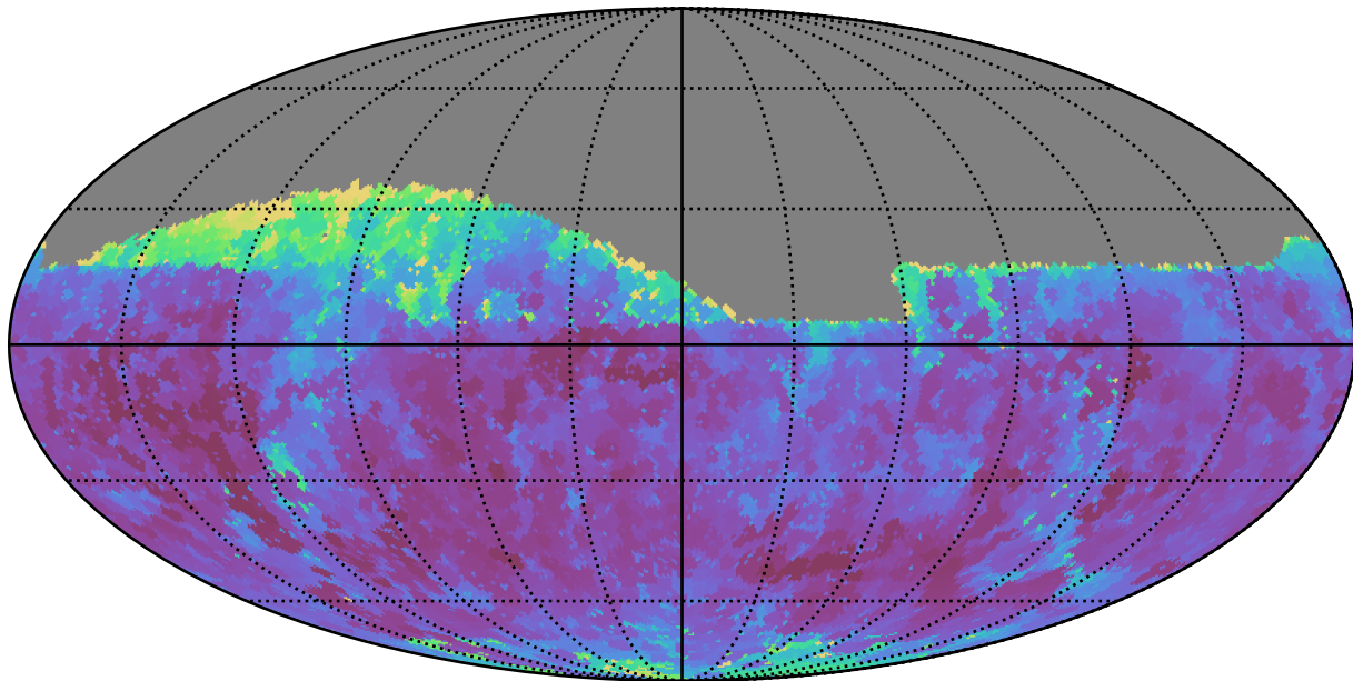
ddf_half_v3.4_10yrs Yr 1 z band: Min seeingEff
