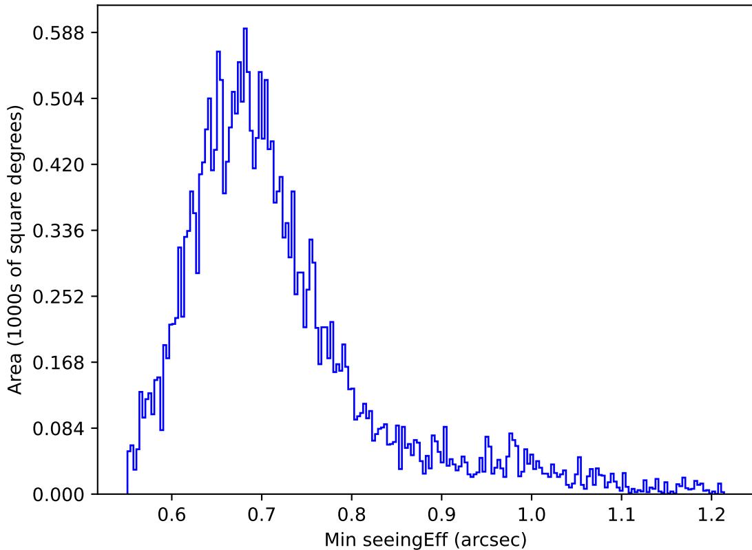
ddf_half_v3.4_10yrs Yr 1 z band: Min seeingEff
