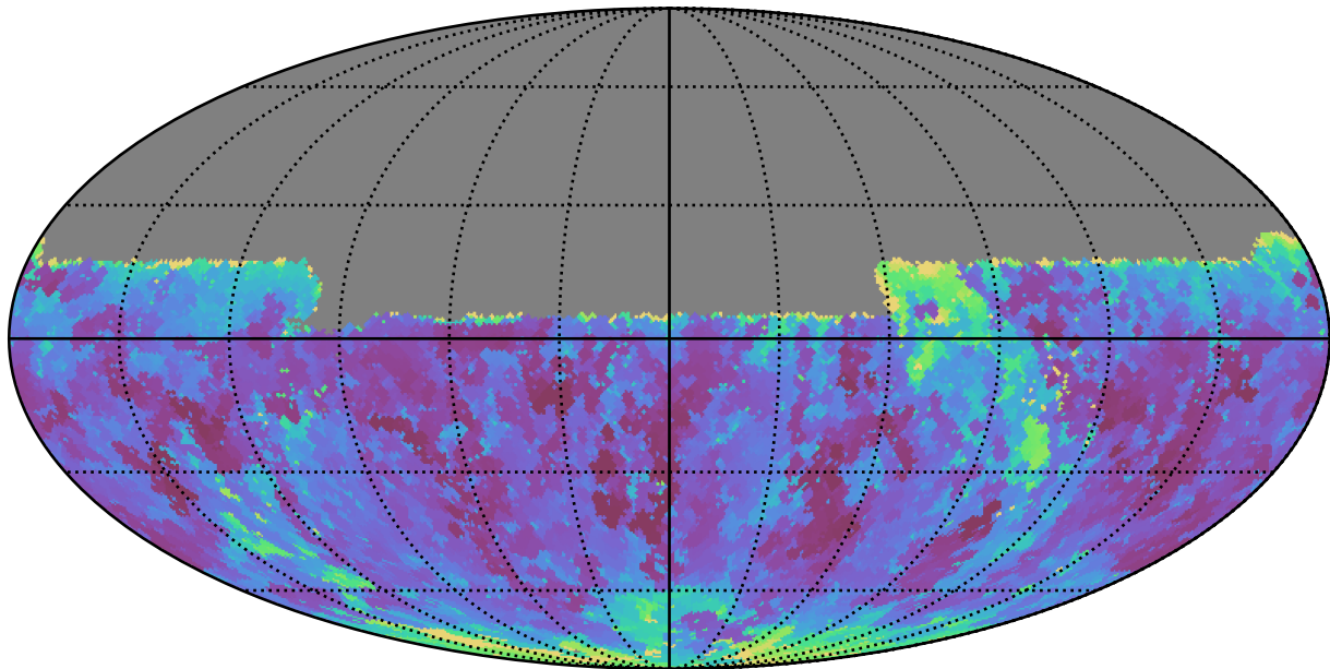
ddf_half_v3.4_10yrs Yr 1 y band: Min seeingEff
