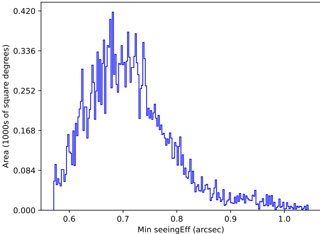
ddf_half_v3.4_10yrs Yr 1 y band: Min seeingEff
