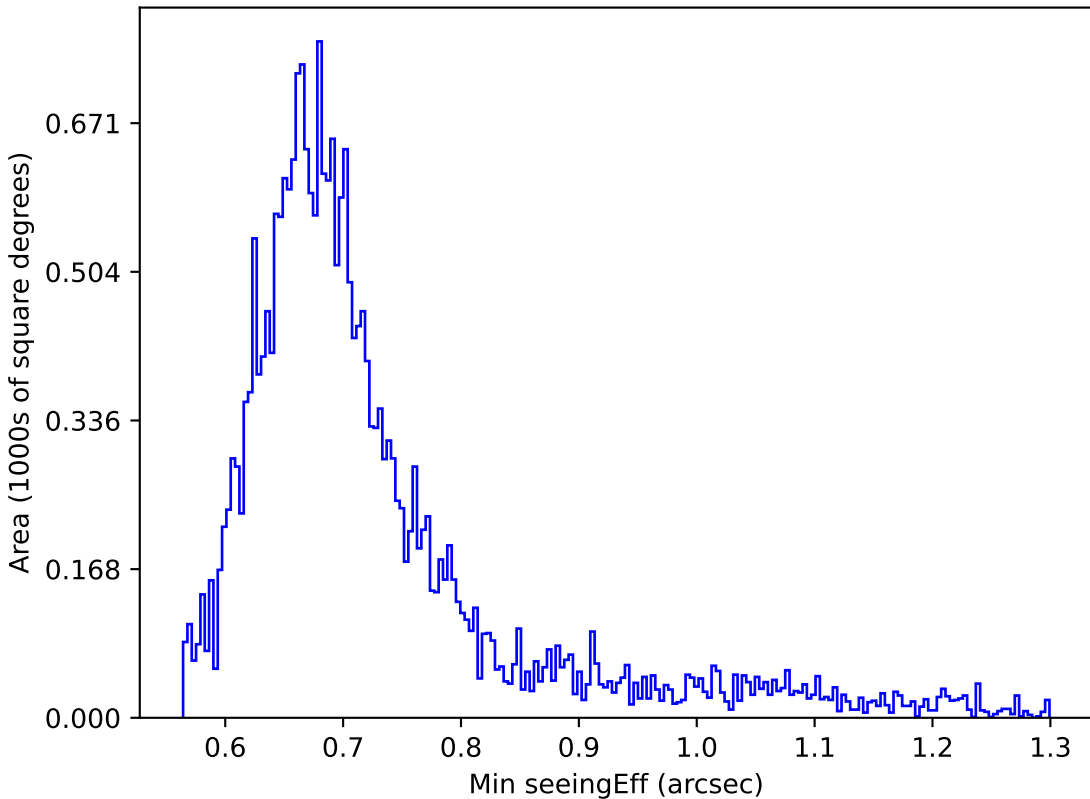
ddf_half_v3.4_10yrs Yr 1 r band: Min seeingEff
