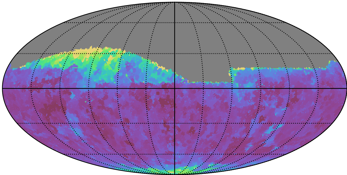
ddf_half_v3.4_10yrs Yr 1 i band: Min seeingEff
