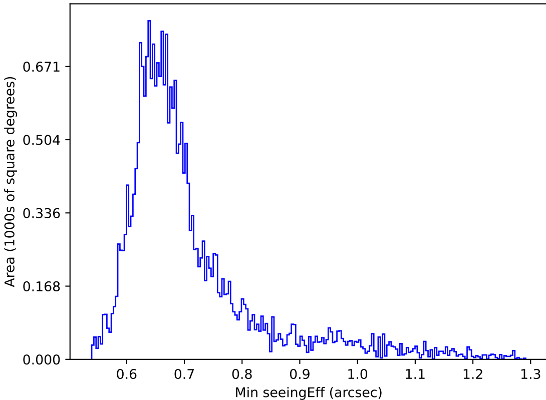
ddf_half_v3.4_10yrs Yr 1 i band: Min seeingEff
