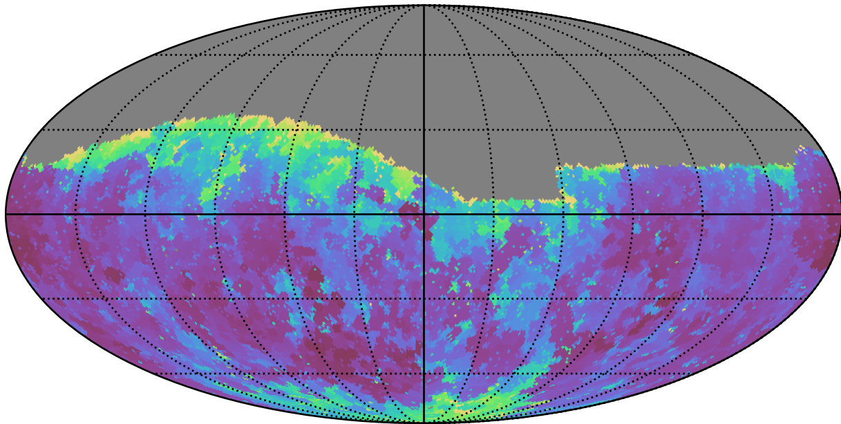
ddf_half_v3.4_10yrs Yr 1 g band: Min seeingEff
