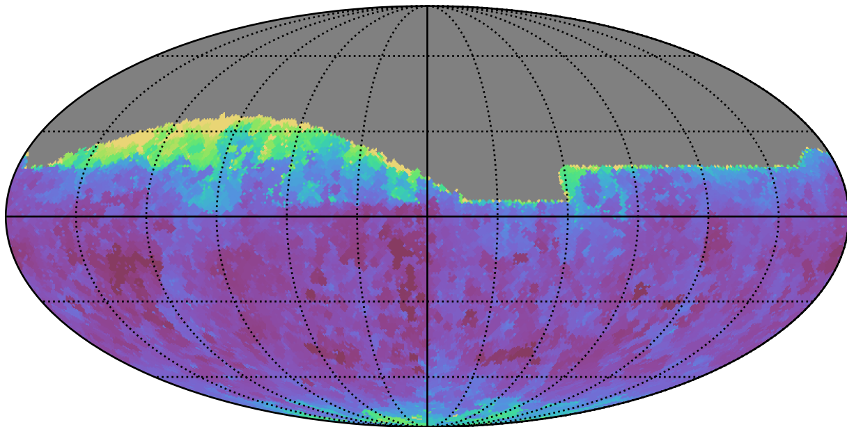
ddf_half_v3.4_10yrs Yr 1 all bands: Min seeingEff
