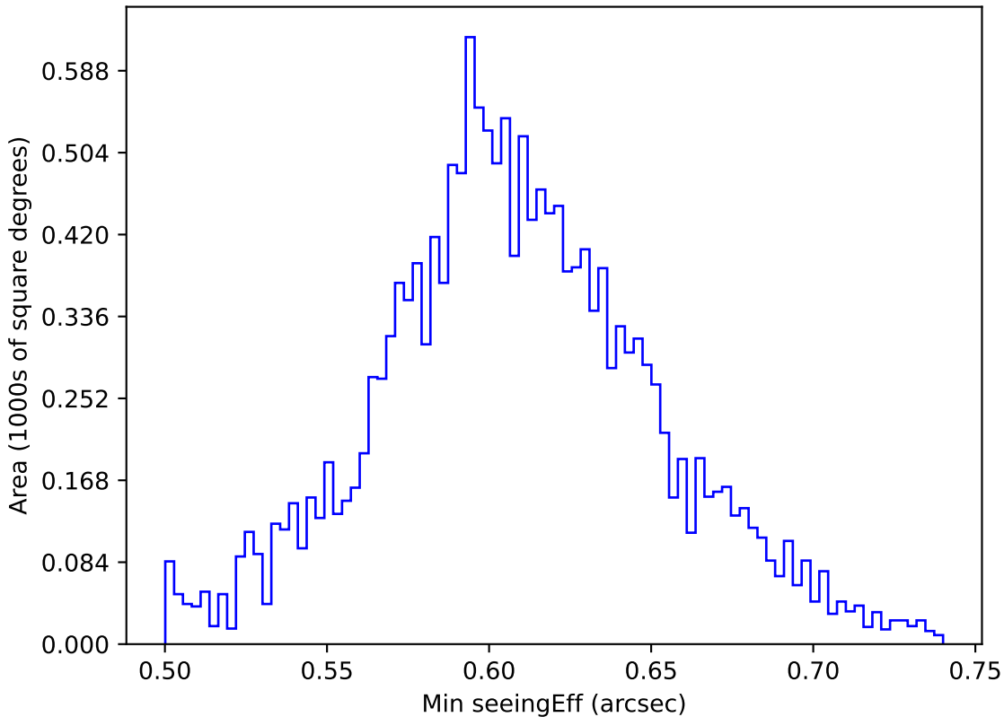
ddf_half_v3.4_10yrs WFD z band: Min seeingEff
