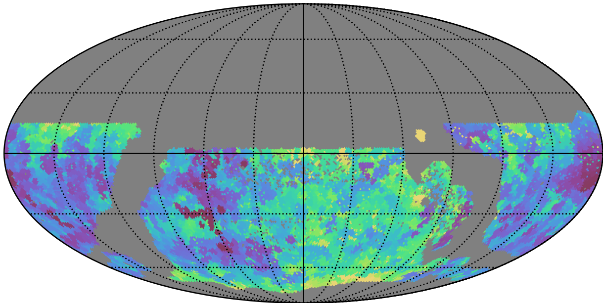
ddf_half_v3.4_10yrs WFD u band: Min seeingEff
