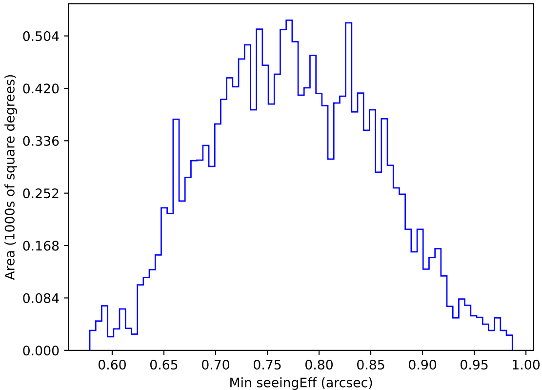
ddf_half_v3.4_10yrs WFD u band: Min seeingEff
