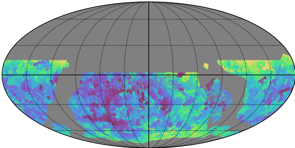
ddf_half_v3.4_10yrs WFD r band: Min seeingEff
