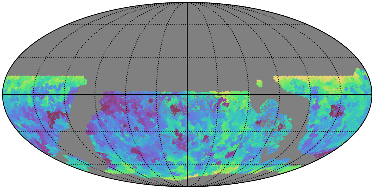
ddf_half_v3.4_10yrs WFD i band: Min seeingEff
