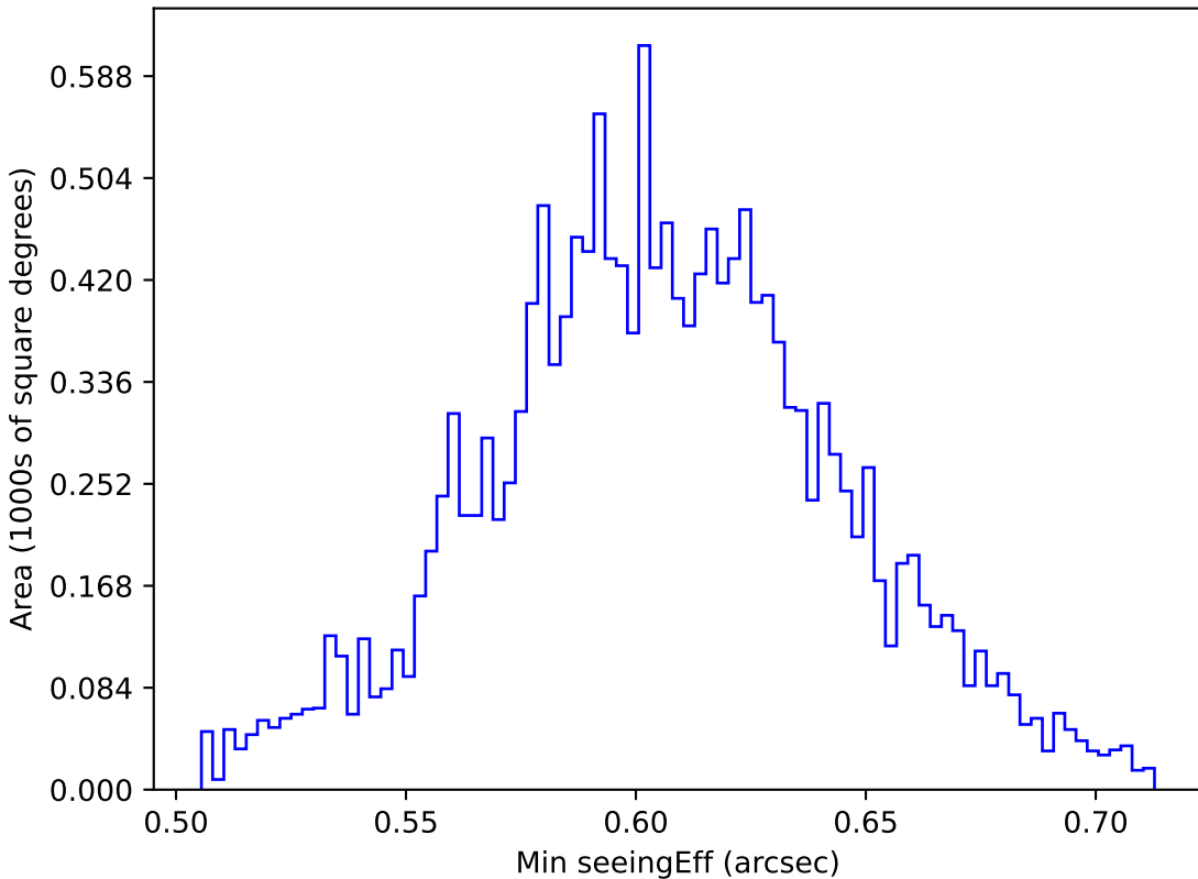
ddf_half_v3.4_10yrs WFD i band: Min seeingEff
