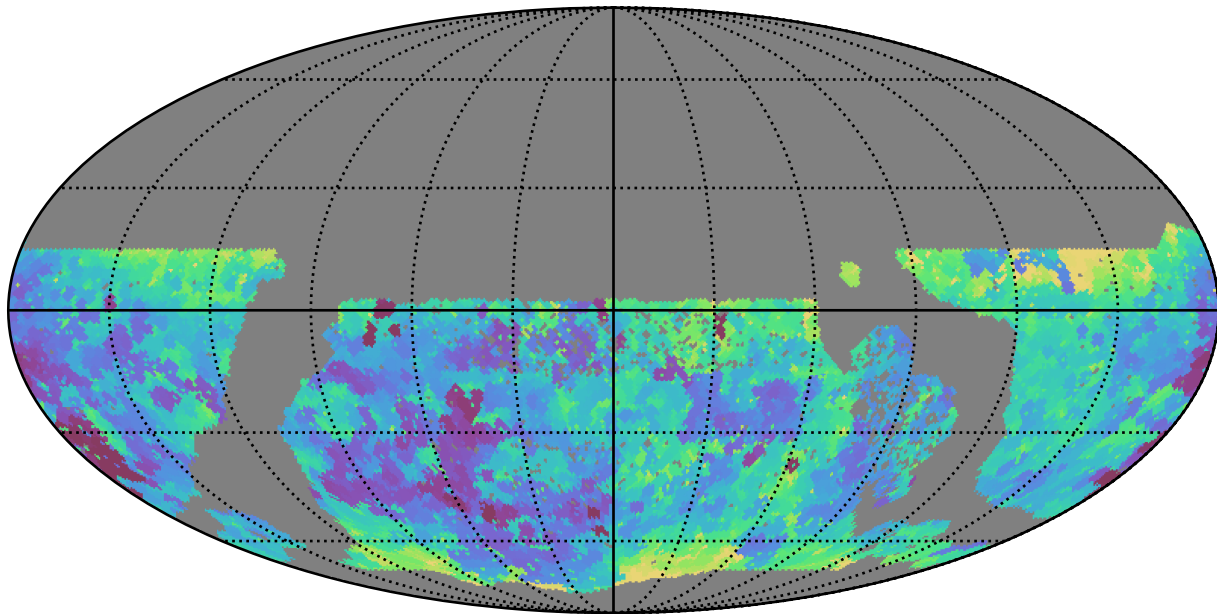
ddf_half_v3.4_10yrs WFD g band: Min seeingEff
