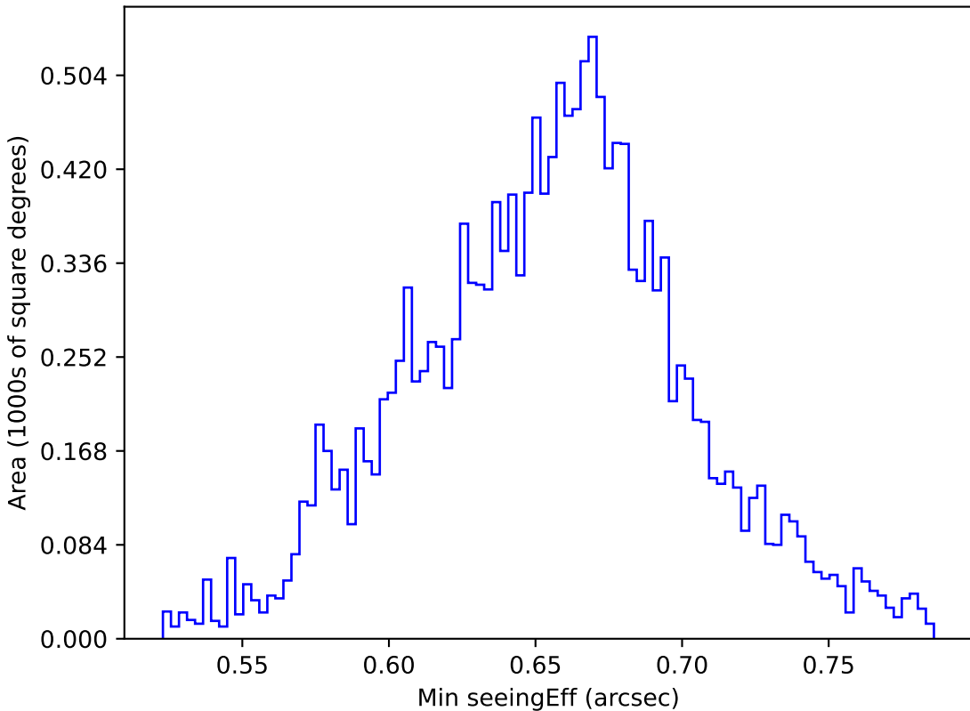
ddf_half_v3.4_10yrs WFD g band: Min seeingEff
