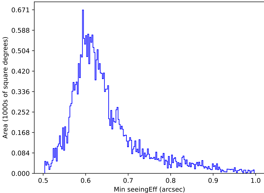
ddf_half_v3.4_10yrs All sky z band: Min seeingEff
