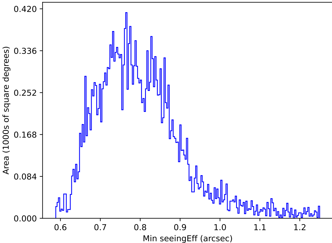
ddf_half_v3.4_10yrs All sky u band: Min seeingEff
