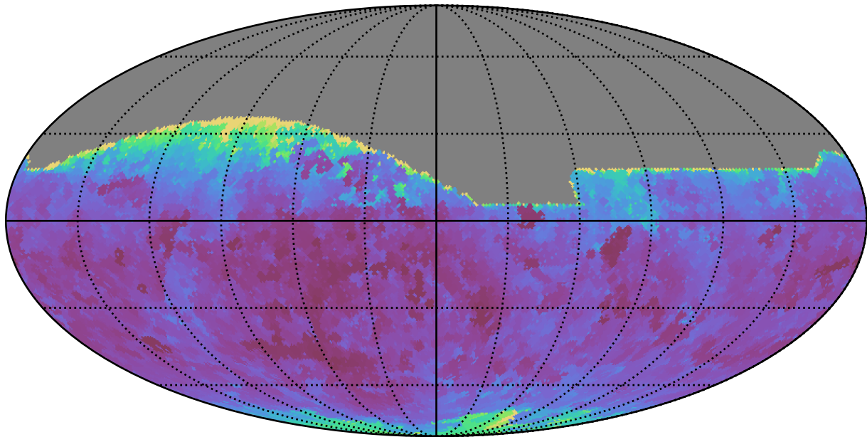
ddf_half_v3.4_10yrs All sky r band: Min seeingEff
