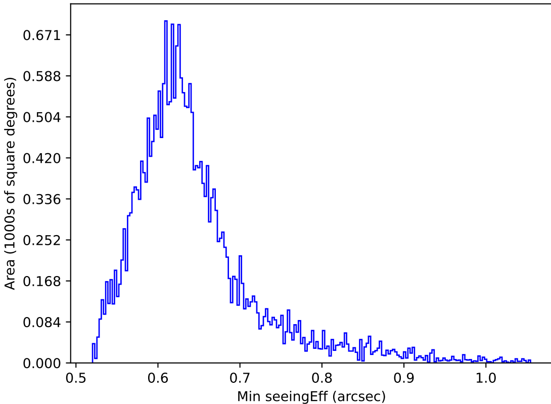
ddf_half_v3.4_10yrs All sky r band: Min seeingEff
