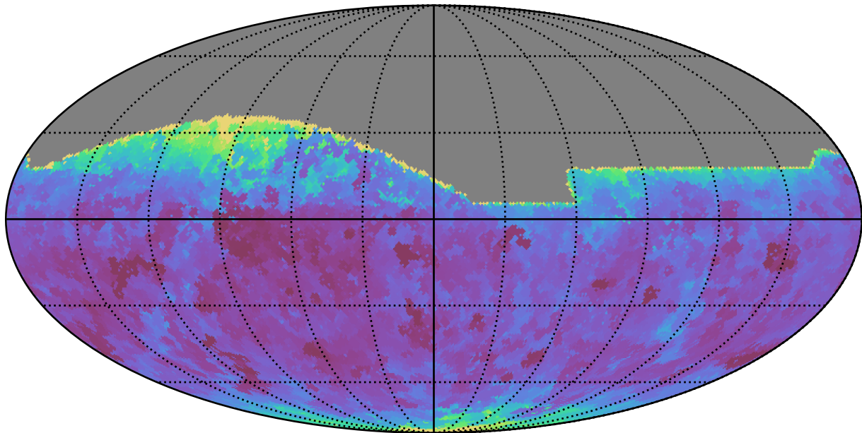
ddf_half_v3.4_10yrs All sky i band: Min seeingEff
