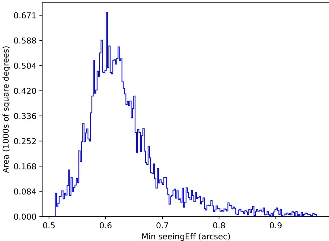
ddf_half_v3.4_10yrs All sky i band: Min seeingEff
