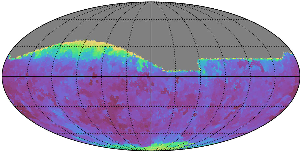
ddf_half_v3.4_10yrs All sky g band: Min seeingEff
