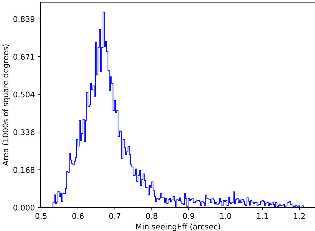
ddf_half_v3.4_10yrs All sky g band: Min seeingEff
