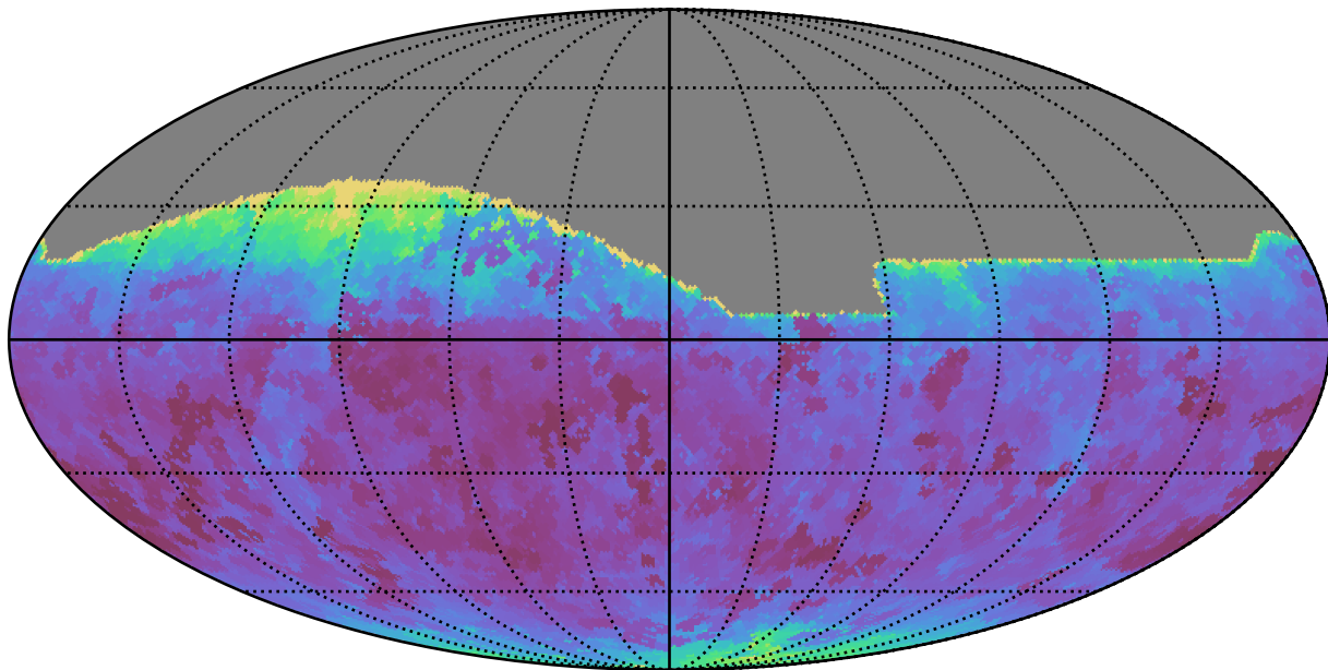
ddf_half_v3.4_10yrs All sky all bands: Min seeingEff
