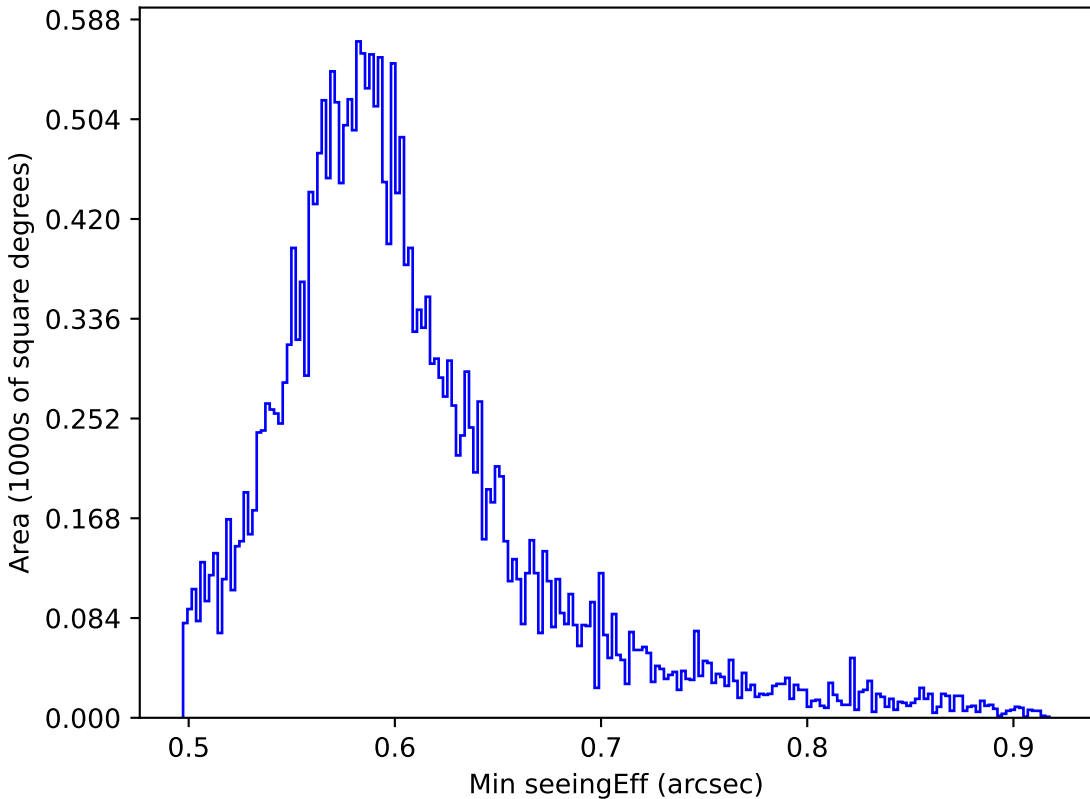
ddf_half_v3.4_10yrs All sky all bands: Min seeingEff
