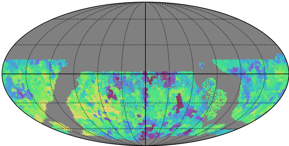
ddf_half_v3.4_10yrs WFD z band: Min saturation_mag
