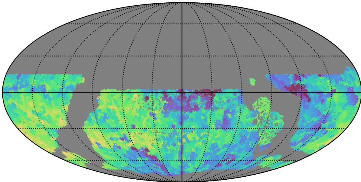
ddf_half_v3.4_10yrs WFD y band: Min saturation_mag
