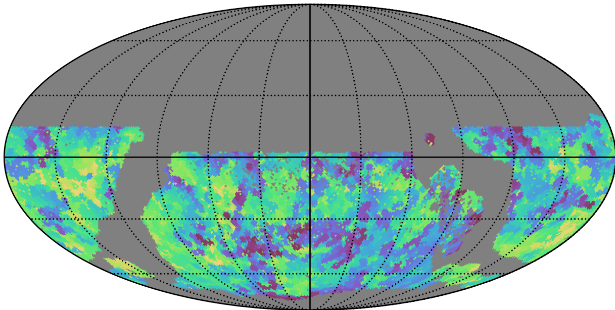
ddf_half_v3.4_10yrs WFD u band: Min saturation_mag
