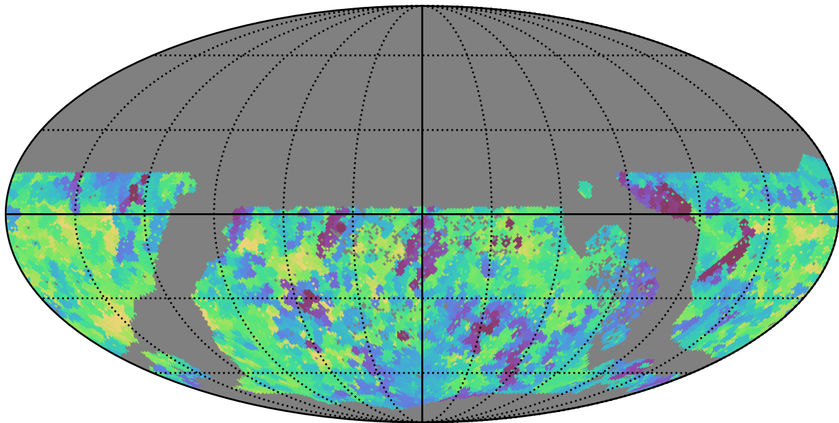
ddf_half_v3.4_10yrs WFD r band: Min saturation_mag
